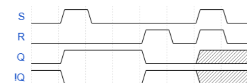
Figure 13: Timing Diagram of an SR-Latch
